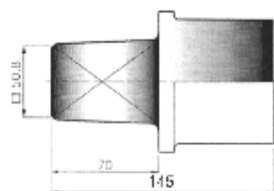
2" Square Nut Adapter
