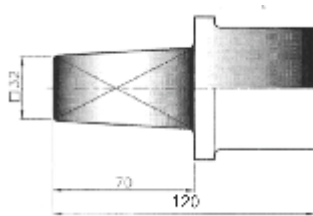
32 Square Nut Adapter
